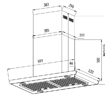
LCH-800I-90SS
